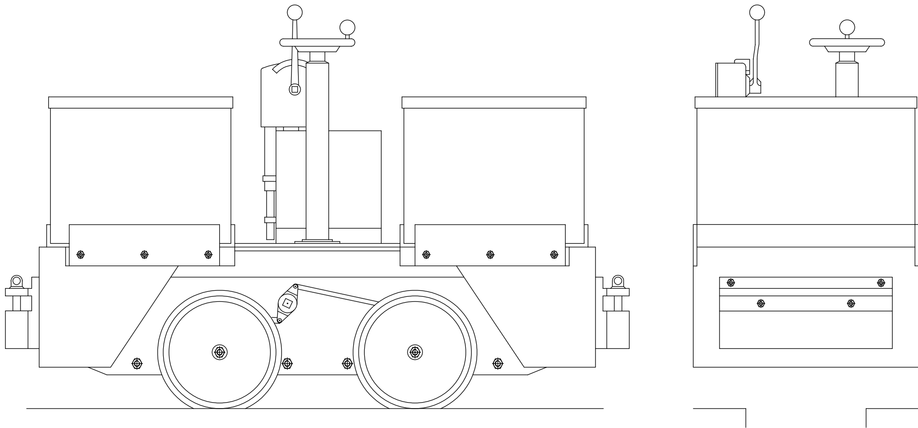
GreenBat originally drawn by Peter Holmes for the book Greenwood & Batley Locomotives 1927-1980 And redrawn to 7/8ths by Ken Cooper May 2007
